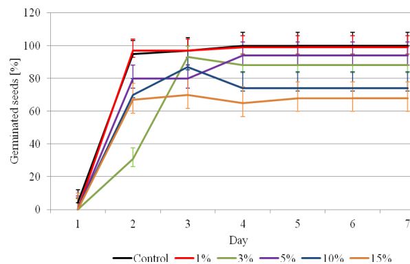
Fig. 1. The influence of the aqueous extracts of the Mentha × piperita L. leaves on the germination of Helianthus annuus L. seeds. Points on lines represent mean value ± SE of 5 replicates
