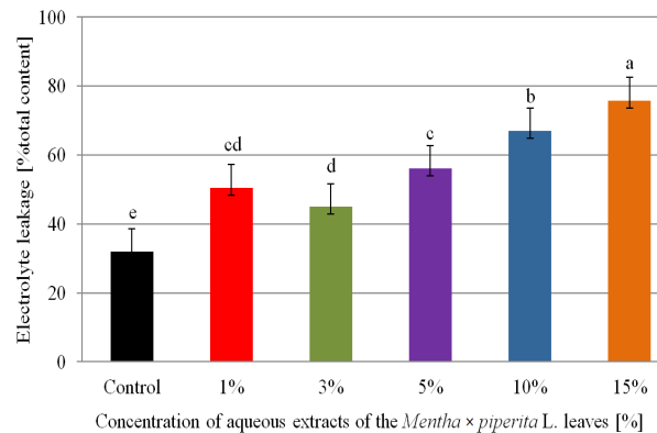
Fig. 2. The influence of aqueous extracts from Mentha × piperita L. leaves on electrolyte leakage from Helianthus annuus L. seedlings, expressed as a percentage of the total electrolyte content in the tissue.
